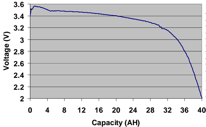
High Temperature Discharge 400mA, 125C
