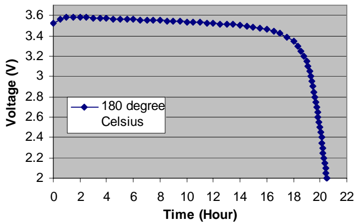
High Temperature Discharge (750mA)
