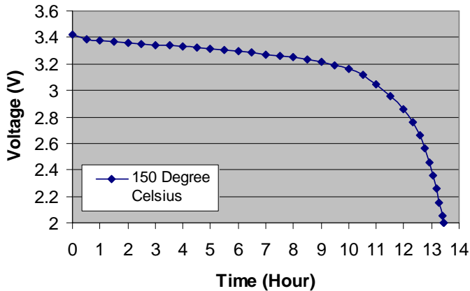
High Temperature Discharge (750mA)
